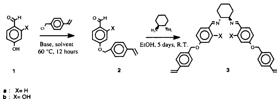
Scheme 1. Synthesis of dialdimine ligands
